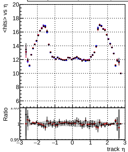
mean hits vs \eta — DQM_original3 — DQM_testMk_initialStepReso — DQM_testMkFitExportFit_initialStepReso
