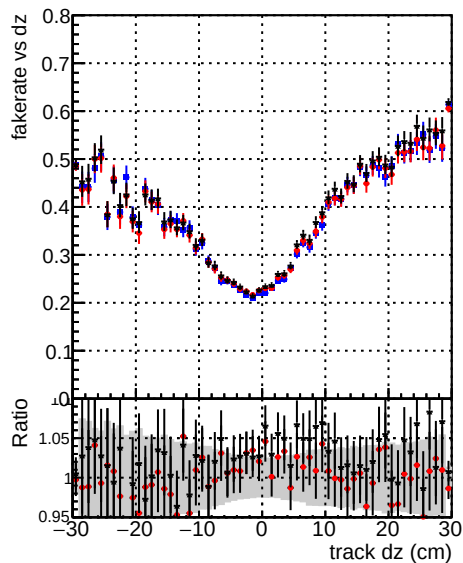
Fake rate vs dz DOM originals DOM testMK DOM FitExport initialStepReso
