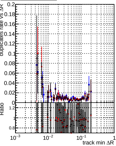
Legend: DQM (blue), testMk (red), testMkFitExportFit (black). Fake rate vs \Delta R (track, jet), Duplicates Rate vs \Delta R (track, jet), Pileup rate vs \Delta R (track, jet).
