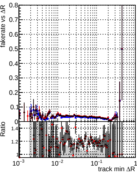
Fake rate vs \Delta R(\text{track, jet}) Legend: \Delta R(\text{track, jet}) (blue line), \Delta R(\text{track, jet}) (red line), \Delta R(\text{track, jet}) (black line)
