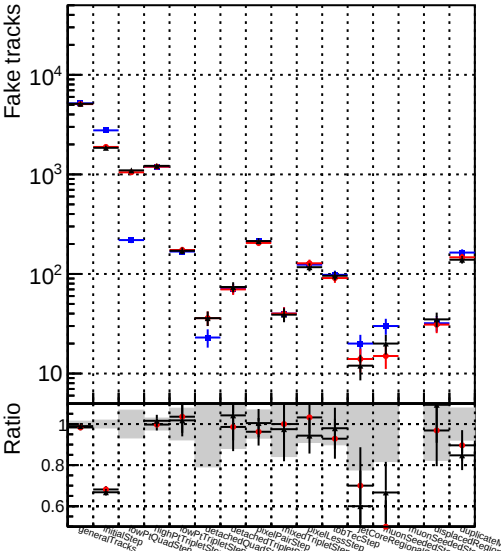
Number —●— DQM_testMk_InitialStepReso —▲— DQM_testMkFitExportFit_initialStepReso
