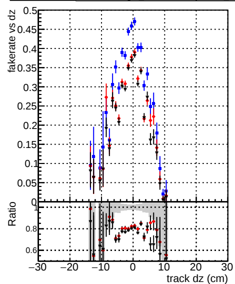
Fake rate vs dz Legend: DOM originals testMK-initialStepReso testMK-FitExport-it-initialStepReso
