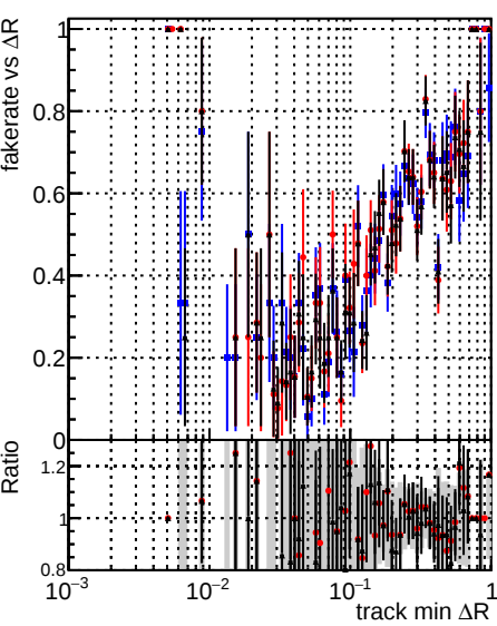
Fake rate vs \Delta R (track, jet) DQM_original3 DQM_testMk_initialStepReso DQM_testMkFitExportFit_initialStepReso
