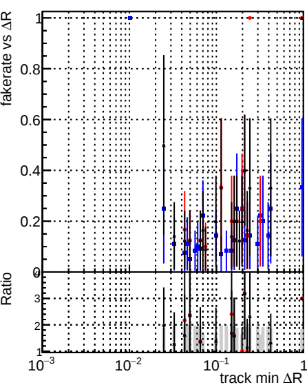
Fake rate vs \Delta R(\text{track, jet}) Legend: DQM_original3 (blue line with dots) DQM_testMk_initialStepReso (red line with dots) DQM_testMkFitExportFit_initialStepReso (black line with dots)
