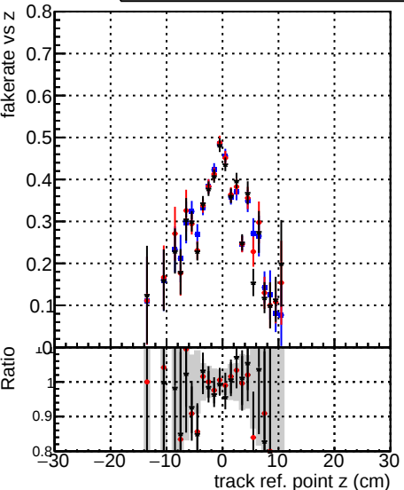
Fake rate vs verpos Legend: DQM_original3 (blue line with dots) DQM_testMk_initialStepReso (red line with dots) DQM_testMkFitExportFit_initialStepReso (black line with dots)
