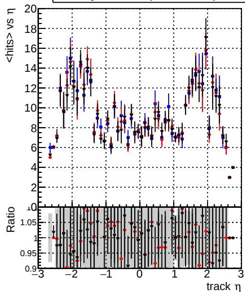
mean hits vs \eta Legend: DQM_original3 (blue line), DQM_testMk_initialStepReso (red line), DQM_testMkFitExportFit_initialStepReso (black line)
