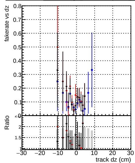
Fake rate vs dz Legend: DOM originals DOM testMK-initialStepReso DOM testMKFitExport-it_initialStepReso
