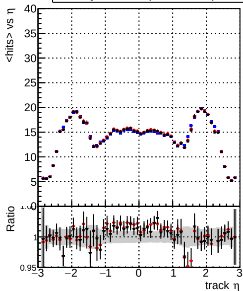
mean hits vs \eta — DQM_original3 — DQM_testMk_initialStepReso — DQM_testMkFitExportFit_initialStepReso
