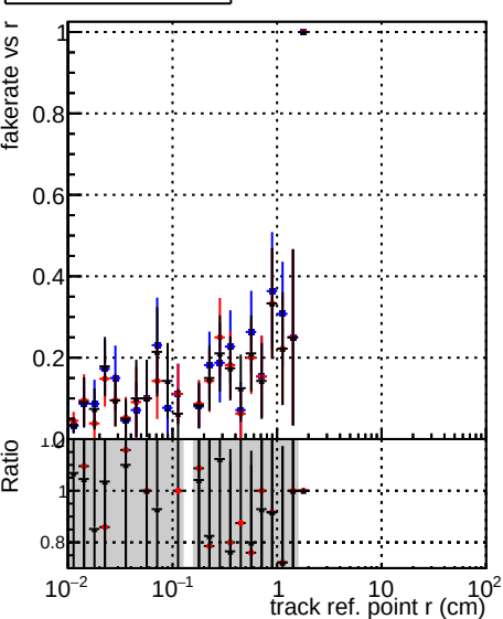
Fake rate vs verpos Duplicates Rate vs verpos Pileup rate vs verpos
