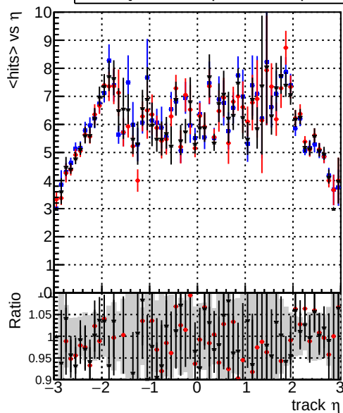
mean hits — DQM_original3 — DQM_testMk_initialStepReso — DQM_testMkFitExportFit_initialStepReso
