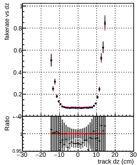
DOM originals DOM testMK-initialStepReso DOM testMKFitExport-it-initialStepReso
