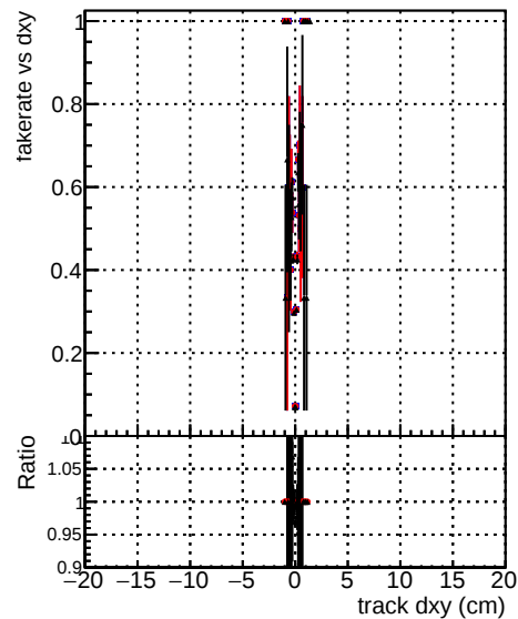
DOM originals DOM testMK-initialStepReso DOM testMKFitExport-it-initialStepReso
