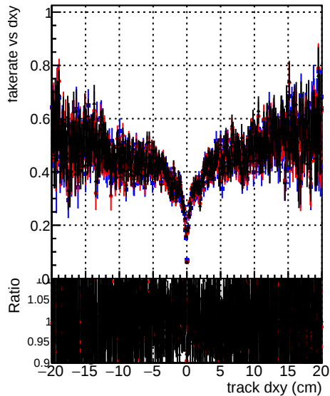
— DOM original — DOM testMK initialStepReso — DOM testMKFitExport initialStepReso
