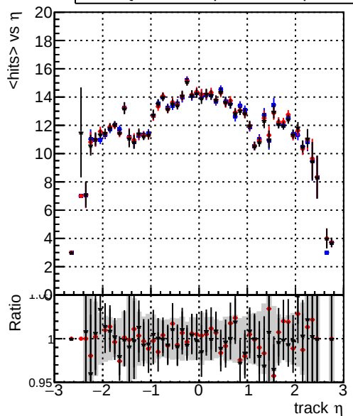
mean hits DQM_original3 DQM_testMk_initialStepReso DQM_testMkFitExportFit_initialStepReso
