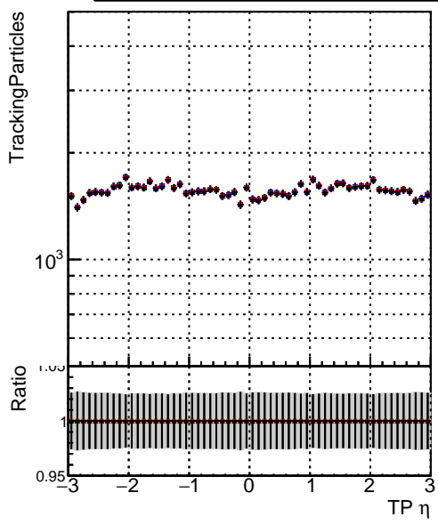
N of simulated tracks vs \eta Legend: DQM_original (blue line with circles) DQM_testMkFitExport_initialStep (red line with circles) DQM_testMkFitExportFit_initialStep (black line with circles)
