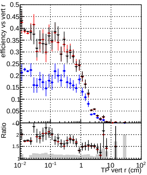
Efficiency vs TP vert r (cm) Legend: DQM_original DQM_testMkFitExport_initialStep DQM_testMkFitExportFit_initialStep
