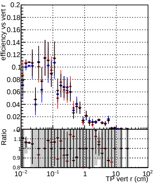
Efficiency vs vertpos Legend: DQM_original DQM_testMkFitExport_initialStep DQM_testMkFitExportFit_initialStep
