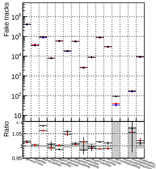
Number of tracks vs collection Legend: DQM_original (Blue line with circles) DQM_testMkFitExport_initialStep (Red line with circles) DQM_testMkFitExportFit_initialStep (Black line with circles)
