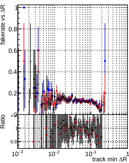
Fake rate vs \Delta R (track, jet) Legend: - \Delta R original (blue line with dots) - \Delta R testMkFitExport_initialStep (red line with dots) - \Delta R testMkFitExportFit_initialStep (black line with dots)
