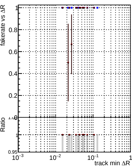
Fake rate vs \Delta R(\text{track, jet}) Legend: DQM_original (blue line with dots) DQM_testMkFitExport_initialStep (red line with dots) DQM_testMkFitExportFit_initialStep (black line with dots)
