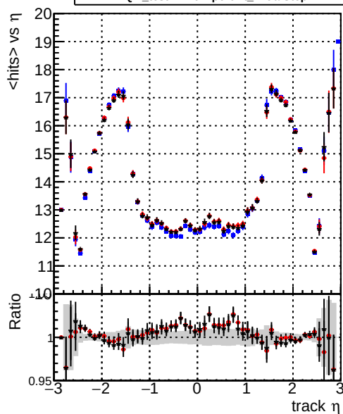
DQM_original DQM_testMkFitExport_initialStep DQM_testMkFitExportFit_initialStep mean hit
