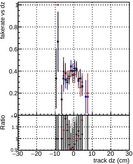
Fake rate vs dz DOM original DOM testMKFitExportFit_initialStep
