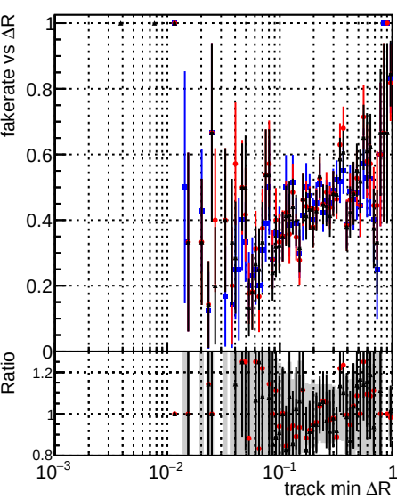
Fake rate vs \Delta R (track, jet) Legend: DQM original (blue line with dots) DQM testMkFitExport_initialStep (red line with dots) DQM testMkFitExportFit_initialStep (black line with dots)
