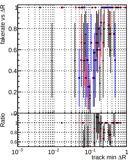
Legend: DQM original (blue), DQM testMkFitExport_initialStep (red), DQM testMkFitExportFit_initialStep (black)
