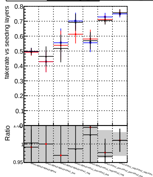
Fake rate vs. DOM original DOM test DOM test MKFitExportFit initialStep
