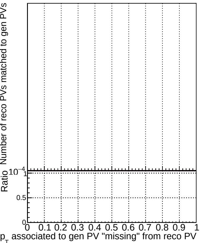
RecoPVAssoc2GenPVMatched_missing
