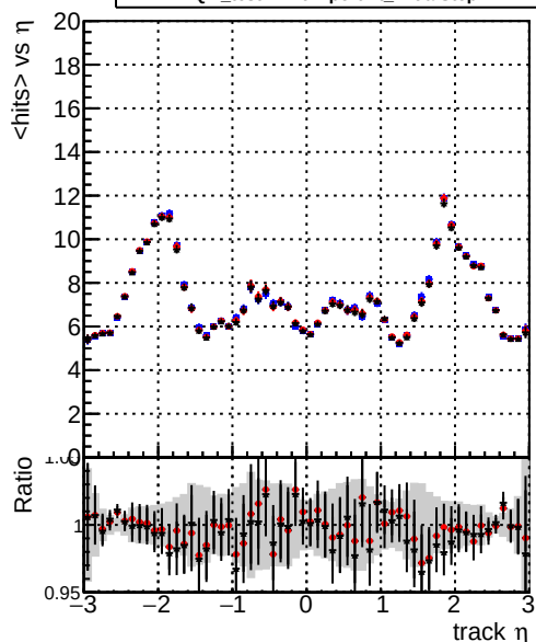
mean hit — DQM_original — DQM_testMkFitExport_initialStep — DQM_testMkFitExportFit_initialStep
