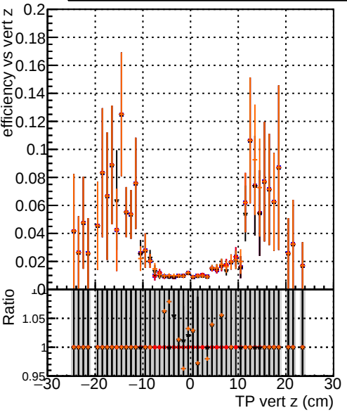
Efficiency vs vertpos —•— DQM_original —•— DQM_original2 —•— DQM_testMkFitExport_initialStep —•— DQM_testMkFitExportFit_initialStep
