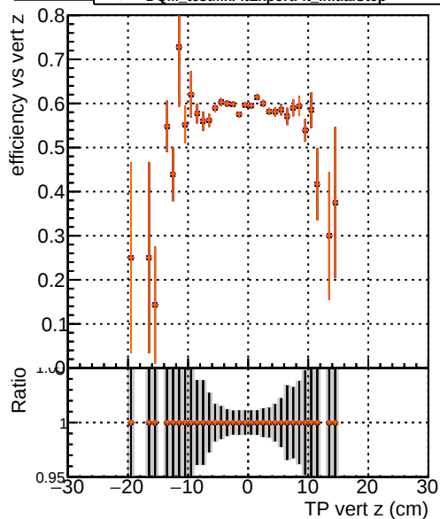
Efficiency vs. sim PV z DOM_original DOM_original2 DOM_testMkFitExport_initialStep DOM_testMkFitExportFit_initialStep
