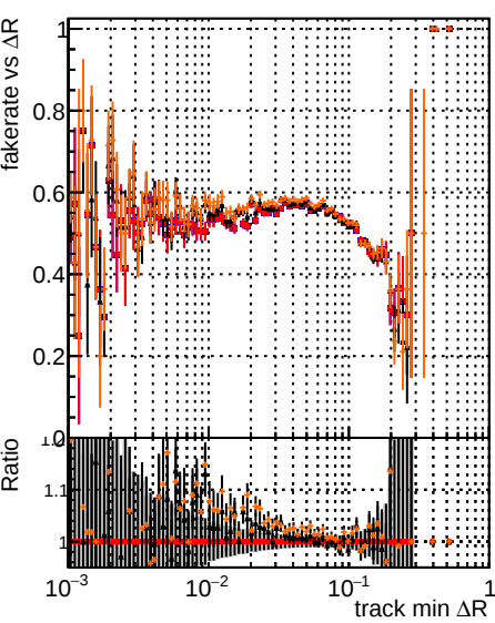
Fake rate vs \Delta R(\text{track, jet}) Legend: DOM original DOM original2 DOM testMKFitExport_initialStep DOM testMKFitExport_fit_initialStep
