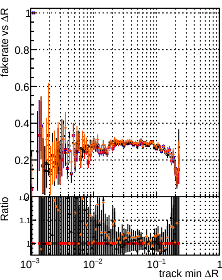
Fake rate vs \Delta R(\text{track, jet}) Legend: DOM original DOM original2 DOM test DOM testMKFitExport_initialStep
