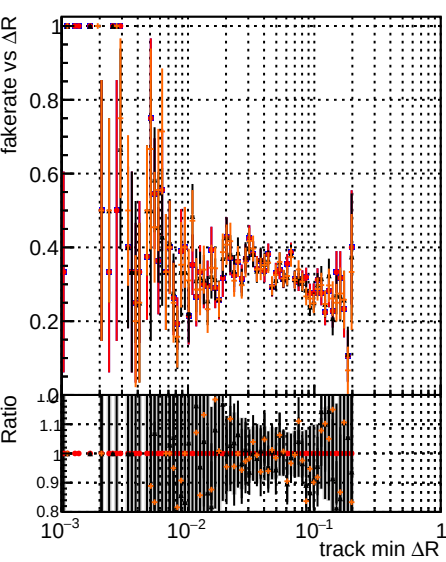
Fake rate vs \Delta R (track, jet) Legend: DOM original DOM original2 DOM testMKFitExport_initialStep DOM testMKFitExport_fit_initialStep
