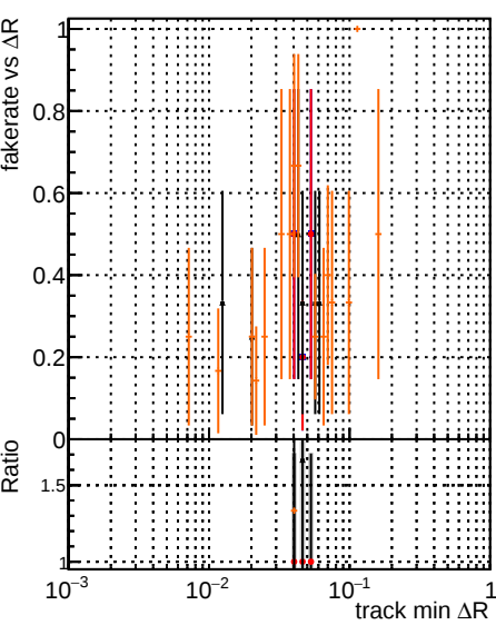
Fake rate vs ΔR(track, jet) Legend: DOM original DOM original2 DOM testMKFitExport_initialStep DOM testMKFitExport_fit_initialStep
