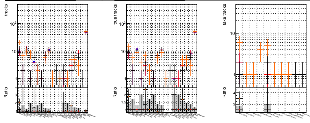
N of reco track vs. \chi^2 BGM original BGM Export-InitialStep BGM testMKFitExport-InitialStep
