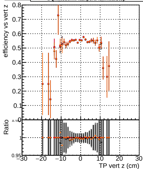
Efficiency vs. TP vert z (cm) Legend: - —•— DQM_original - —•— DQM_original2 - —•— DQM_testMkFitExport_initialStep - —•— DQM_testMkFitExportFit_initialStep
