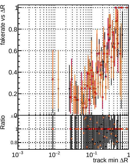
Fake rate vs ΔR(track, jet) Legend: DOM original DOM original2 DOM testIMkFitExport_initialStep DOM testIMkFitExport_initialStep
