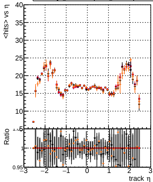
mean hit Legend: DQM_original (blue line with circles), DQM_original2 (red line with circles), DQM_testMkFitExport_initialStep (black line with circles), DQM_testMkFitExportFit_initialStep (orange line with circles)
