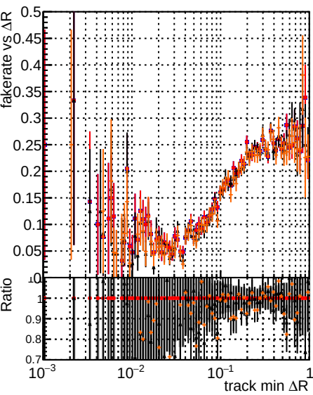
Fake rate vs ΔR(track, jet) Legend: DOM original DOM original2 DOM testMKFitExport_initialStep DOM testMKFitExport_initialStep
