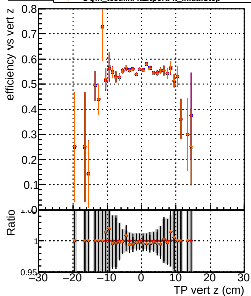
Efficiency vs. TP vert z (cm) Legend: - DQM_original (blue circles) - DQM_original2 (red circles) - DQM_testMkFitExport_initialStep (black circles) - DQM_testMkFitExportFit_initialStep (orange circles)
