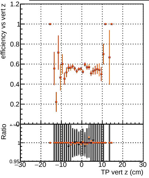
Efficiency vs vert z Legend: DQM_original (blue line with circles) DQM_original2 (red line with circles) DQM_testMkFitExport_initialStep (black line with triangles) DQM_testMkFitExportFit_initialStep (orange line with circles)
