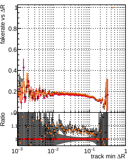
Fake rate vs \Delta R(\text{track, jet}) Legend: DOM original DOM original2 DOM test IMKFit Export initial Step
