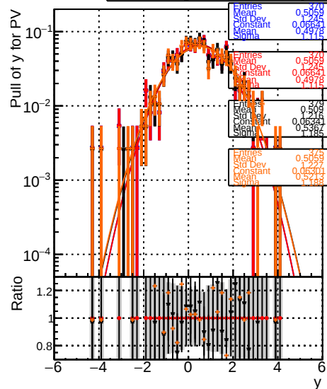
RecoPVAssoc2GenPVMatched_PullY Legend: - Blue line: original - Red line: test - Black line: fit - Orange line: fit initialStep - Grey line: fit initialStep
