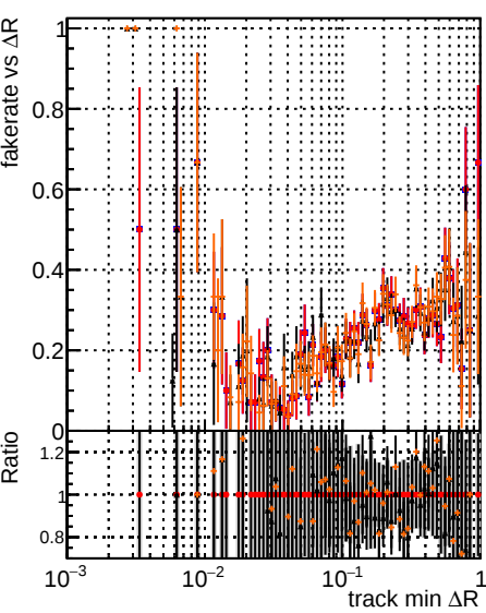
Fake rate vs \Delta R(\text{track, jet}) for DQM original, DQM original2, DQM testMKFitExport_initialStep, and DQM testMKFitExport_initialStep.
