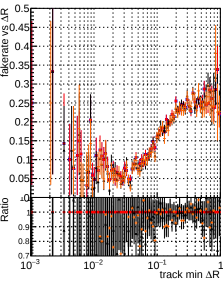
Fake rate vs \Delta R(\text{track, jet}) Legend: DOM original DOM original2 DOM testMKFitExport_initialStep DOM testMKFitExport_initialStep
