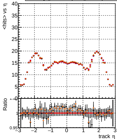
mean hit Legend: DQM_original (blue line), DQM_original2 (red line with dots), DQM_testMkFitExport_initialStep (black line with dots), DQM_testMkFitExportFit_initialStep (orange line with dots)
