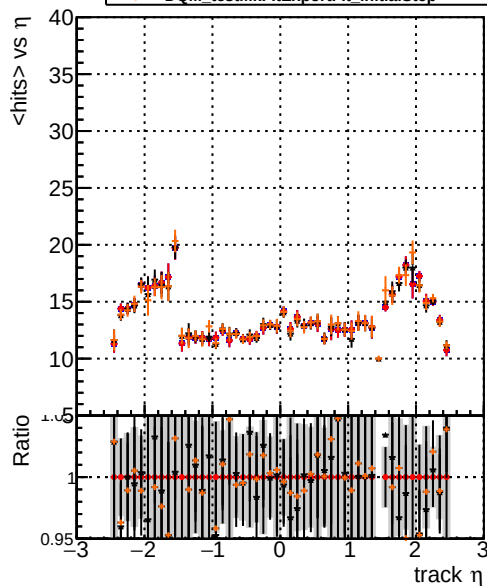
mean hit Legend: Blue line with circles: DQM_original Red line with circles: DQM_original2 Black line with circles: DQM_testMkFitExport_initialStep Orange line with circles: DQM_testMkFitExportFit_initialStep
