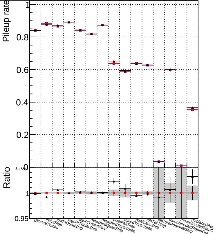
Pileup rate vs collection
